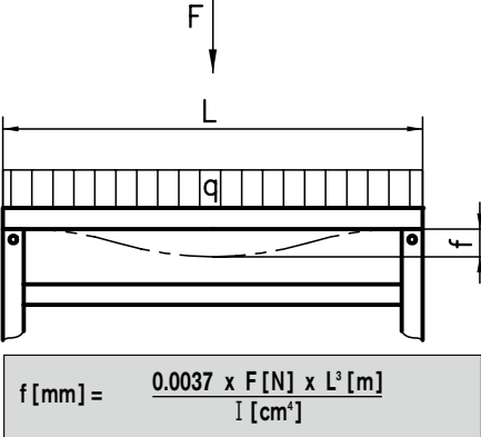
Load case 4
