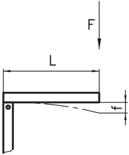
Load case 1
