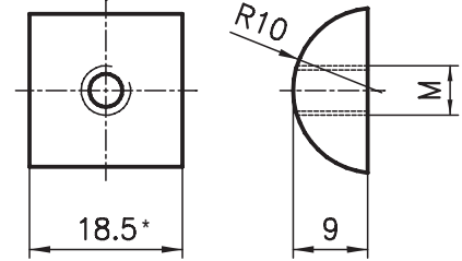
Extrusions base of 50
