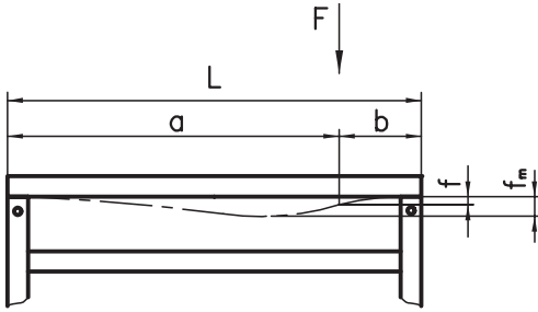
Load case 3
