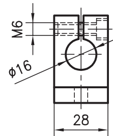
Shaft clamping block - 90°
